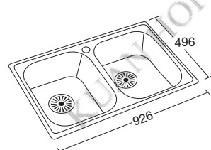
BCM6201T Dimension: 926 x 496 x 220mm Thickness: 1.0mm Installation: Under-mount Material: SUS304 Stainless Steel
